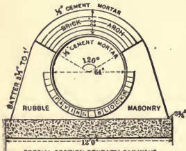
FIG. 8. SALT LAKE CITY, OUTLET SEWER.
